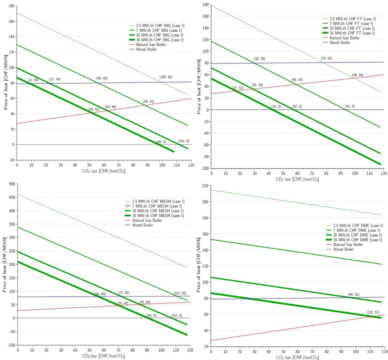
Fig. 5. Case I: CHF (SNG, MEOH, FT and DME) with different plant sizes.
